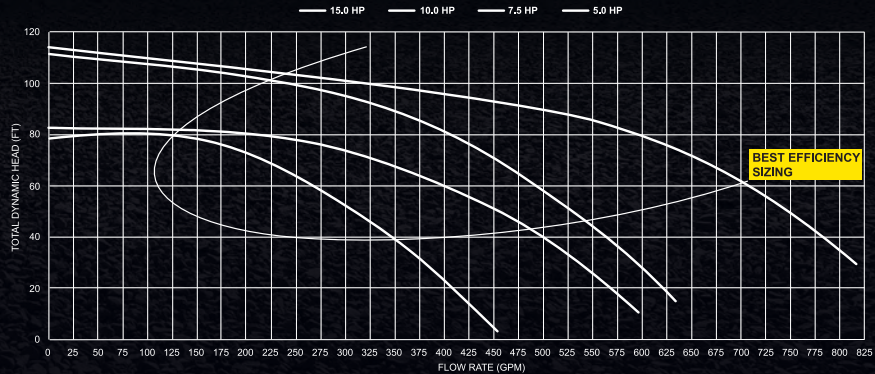
JCP Performance Curves No Strainer
